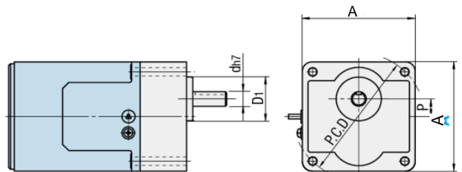
Drive motor dimensions
