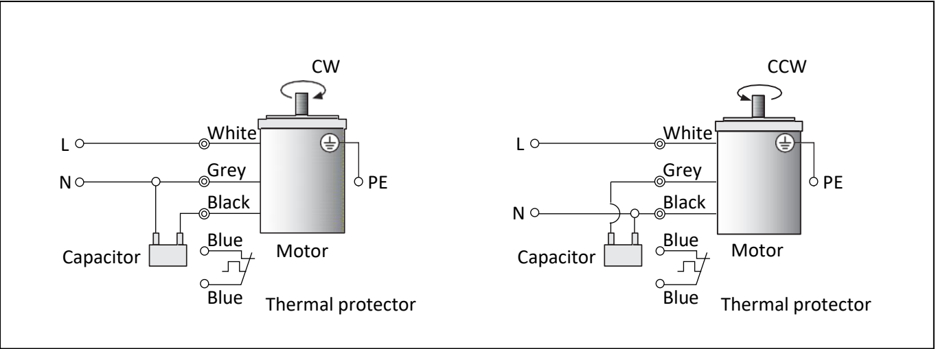
Connection diagram: Induction Motor 6W-25W-40W-60W-90W – 230V/50Hz – 1-phase All motors come with thermal protector except for 6W motor.
