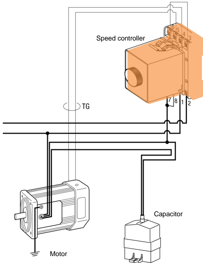
Connection example - motor type with controller
