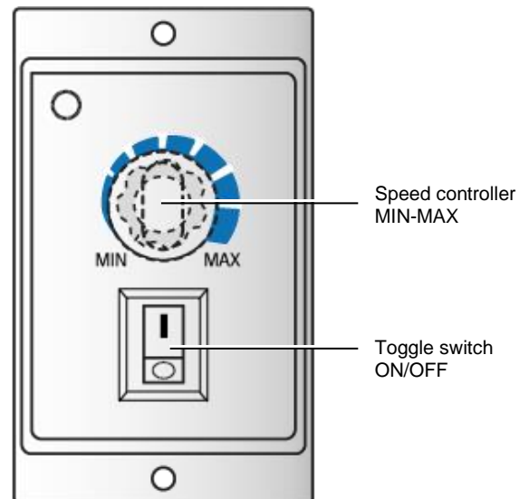
Drive motor speed controller (rail mounting)
