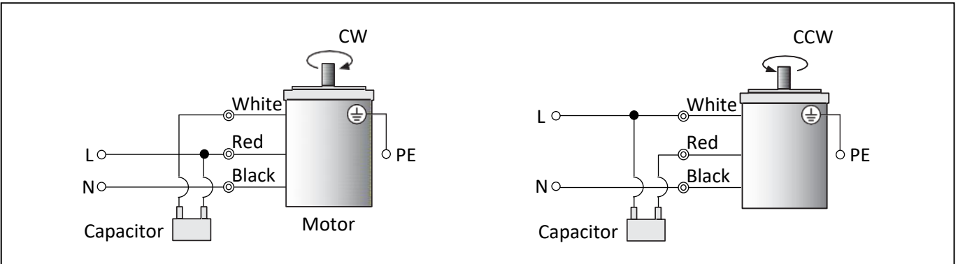
Connection diagram: Induction Motor 6W-25W-40W-60W-90W – 230V/50Hz – 1-phase
