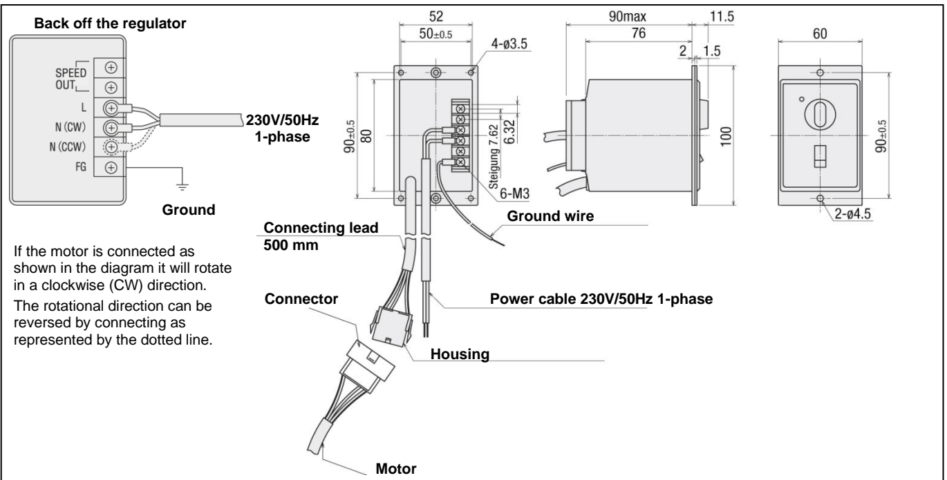
Connection diagram: Variable Speed Motor 6W-25W-40W – 230V/50Hz – 1-phase
