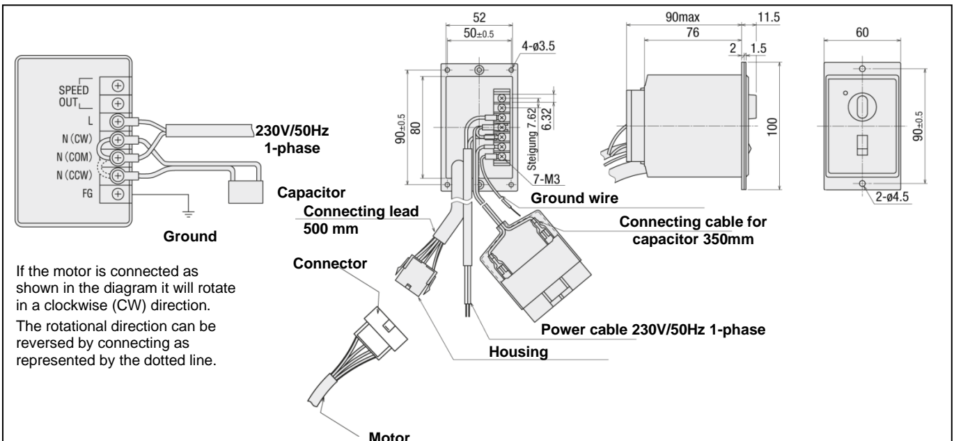
Connection diagram: Variable Speed Motor 60W-90W – 230V/50Hz – 1-phase
