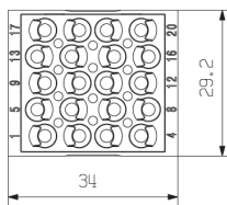
HDC-MHE 20-modules in the IP65-housing, Conductor H05V-K0,5:
